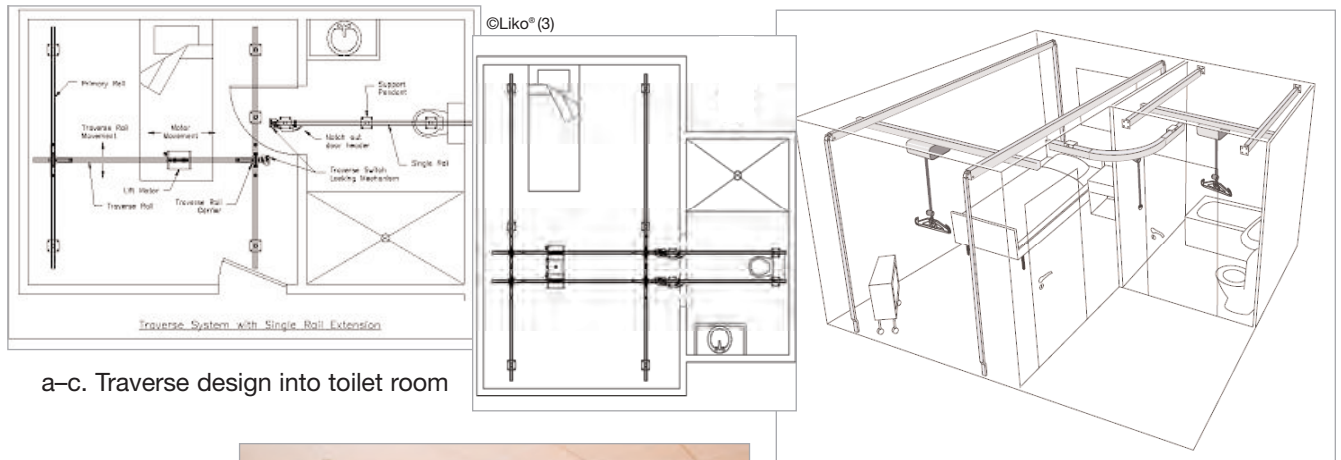
K-5: Ceiling-Lift Tracks Extending from Patient Room into Toilet Room
